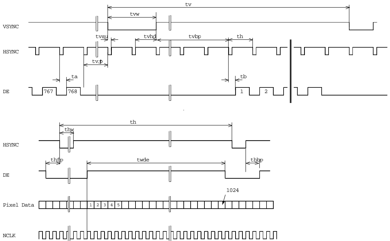
(3) Vertical / Horizontal Sync Timing
